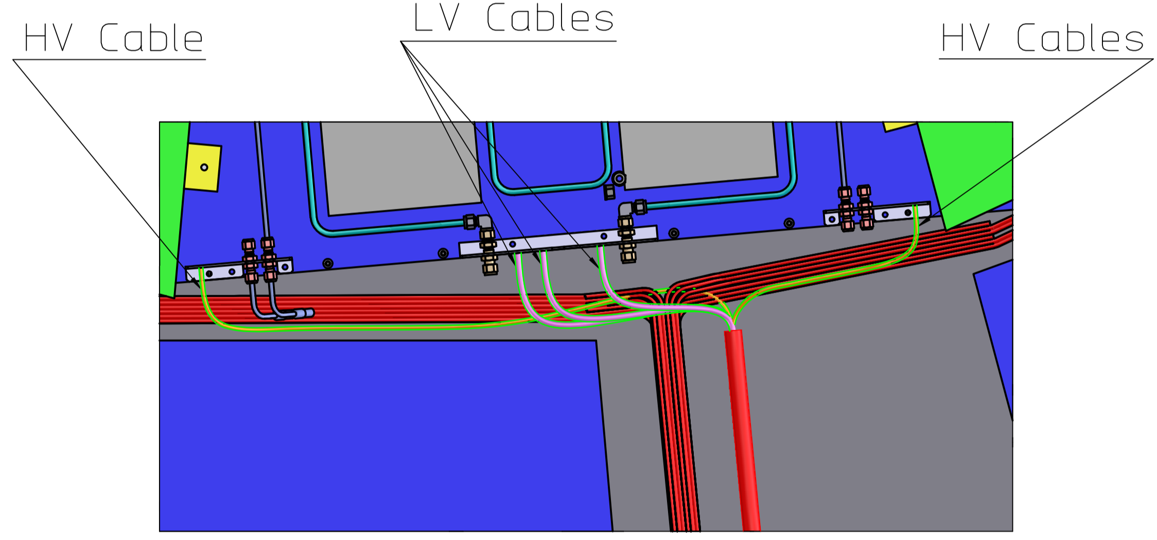
DETAIL7 Scale 1:5
