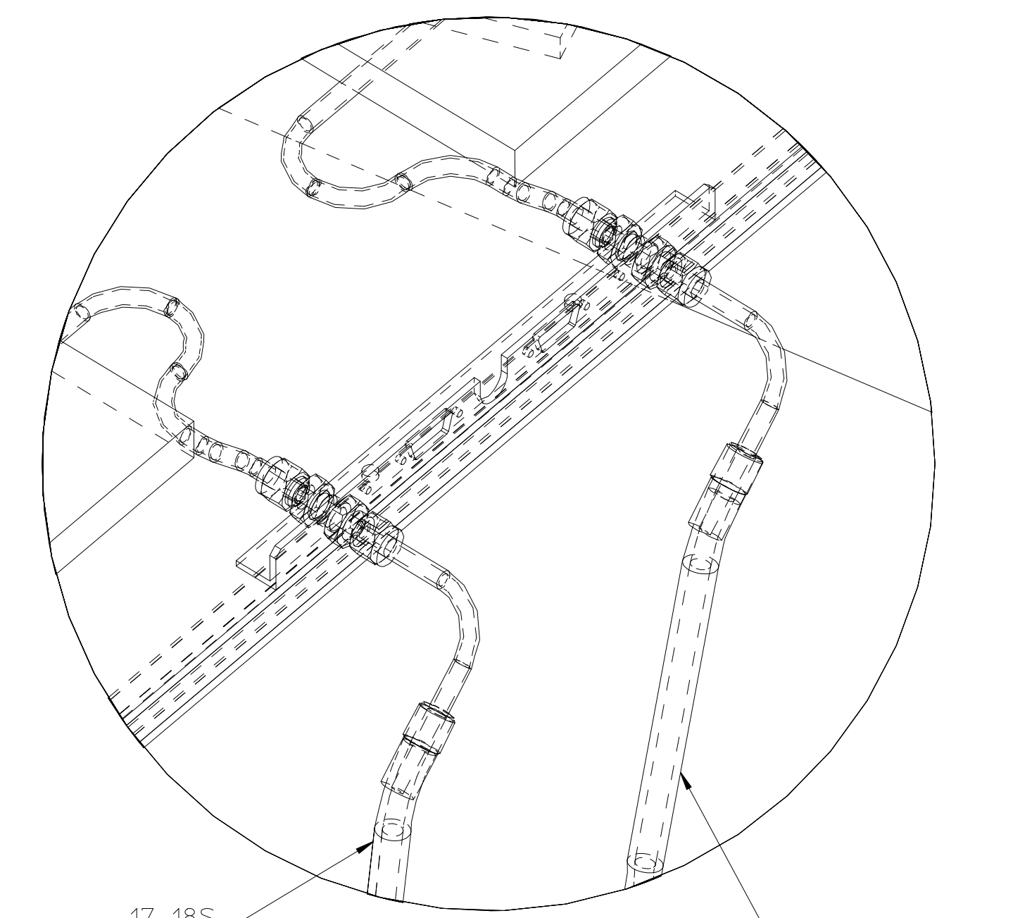
DETAIL18 Scale 1:2
