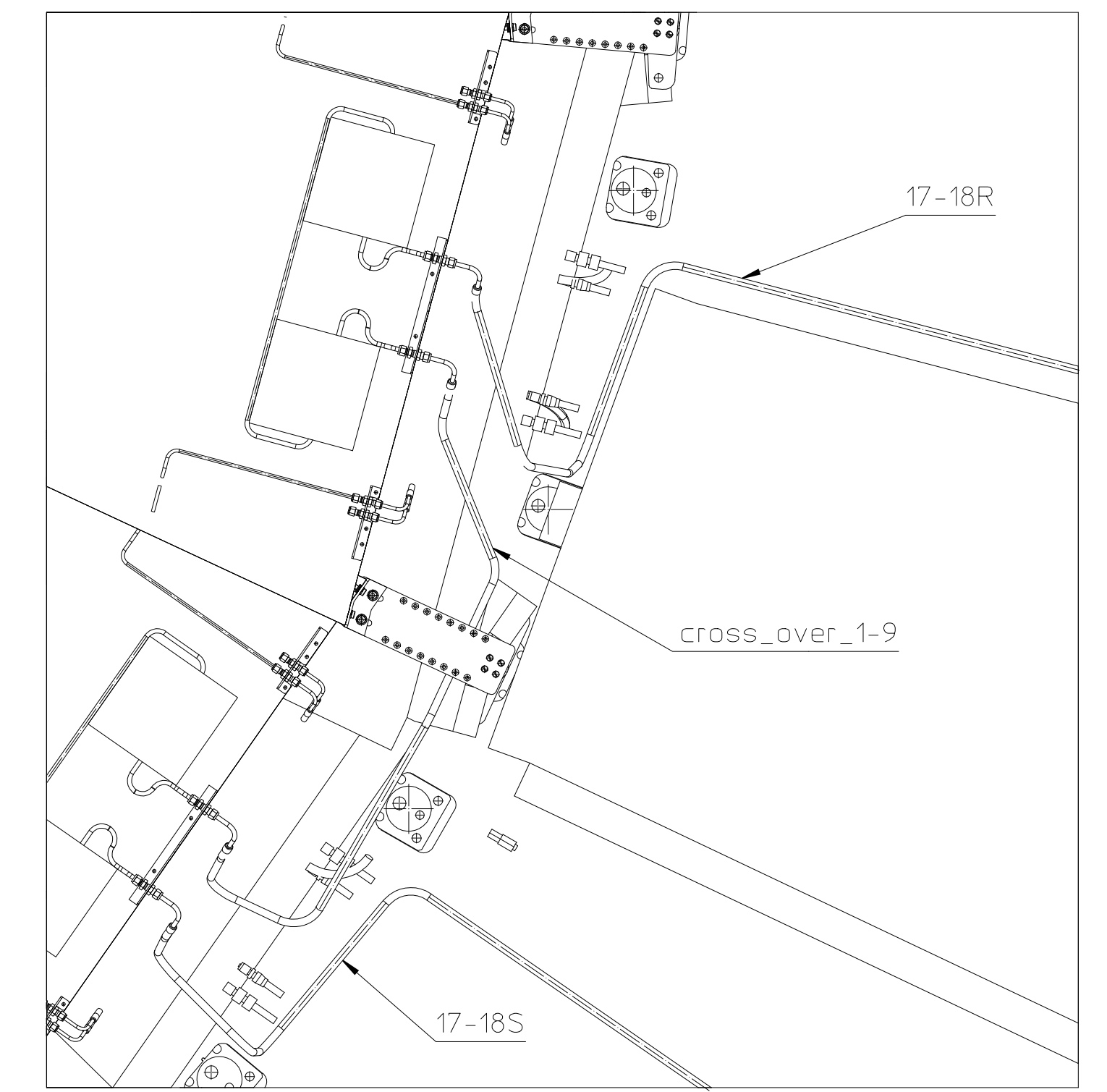
Partial4 Scale 1:10
