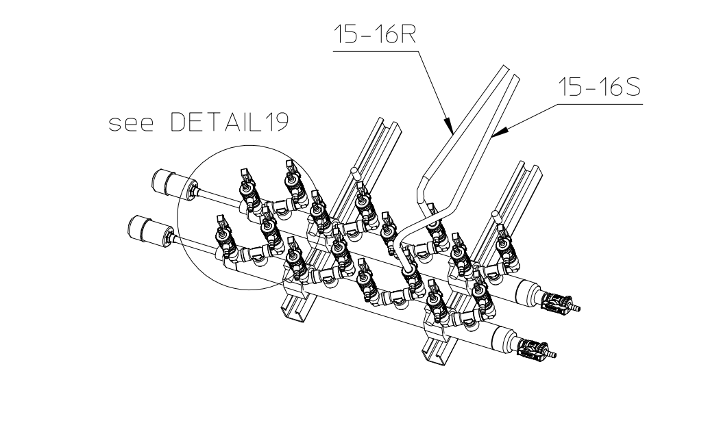
MM 06 DETAIL16 Scale 1:10
