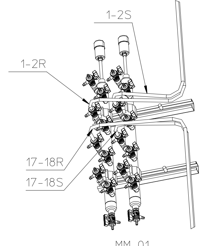
MM 01 DETAIL11 Scale 1:10
