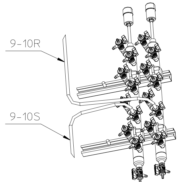
MM 04 DETAIL14 Scale 1:10
