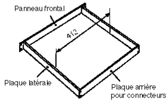
CHASSIS 1 UNITE
