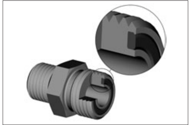
Fig 1 – Captive O-ring Groove (CORG) cutaway
