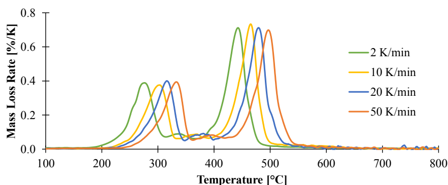
Figure 4. Mass loss rate collected in TGA experiments carried out in nitrogen at heating rates of 2, 10, 20, and 50 K/min.
