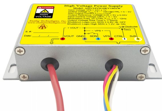
Figure 1.2. Side View
