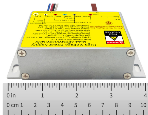
Figure 1.3. Side View
