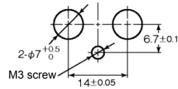
*1. Recommended installation size
