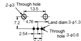
Recommended connector hole size (Back side)
