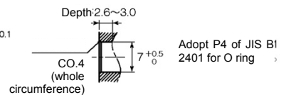
Recommended O ring hole processing size
