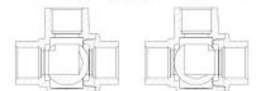
S.76 3-way "L" port operating positions
