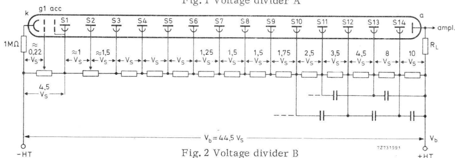
Fig. 2 Voltage divider B
