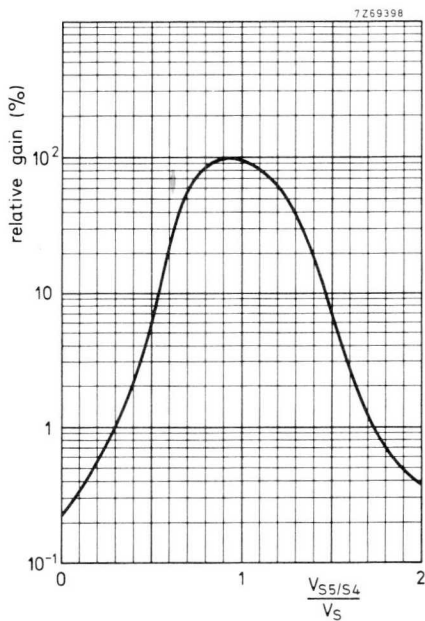
Fig. 7 Relative gain as a function of the voltage between S5 and S4 normalized to V_S V_{S5/S4} constant.
