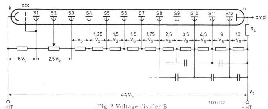
Fig. 2 Voltage divider B
