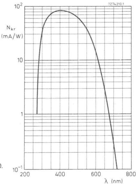
Fig. 6 Spectral sensitivity characteristic XP2020.
