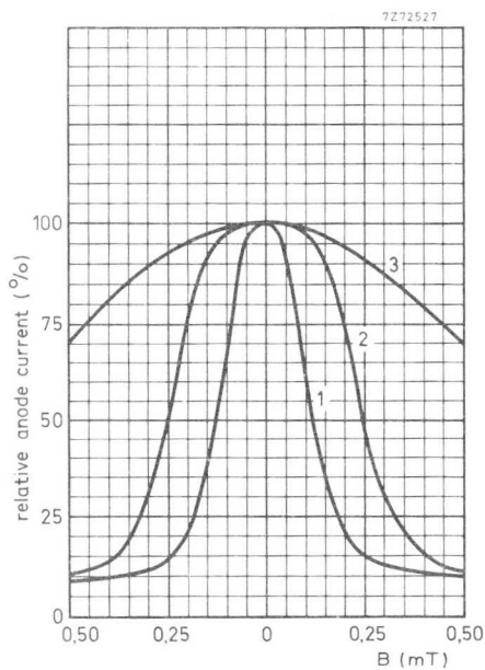
Fig. 4 Relative anode current as a function of the flux density B
