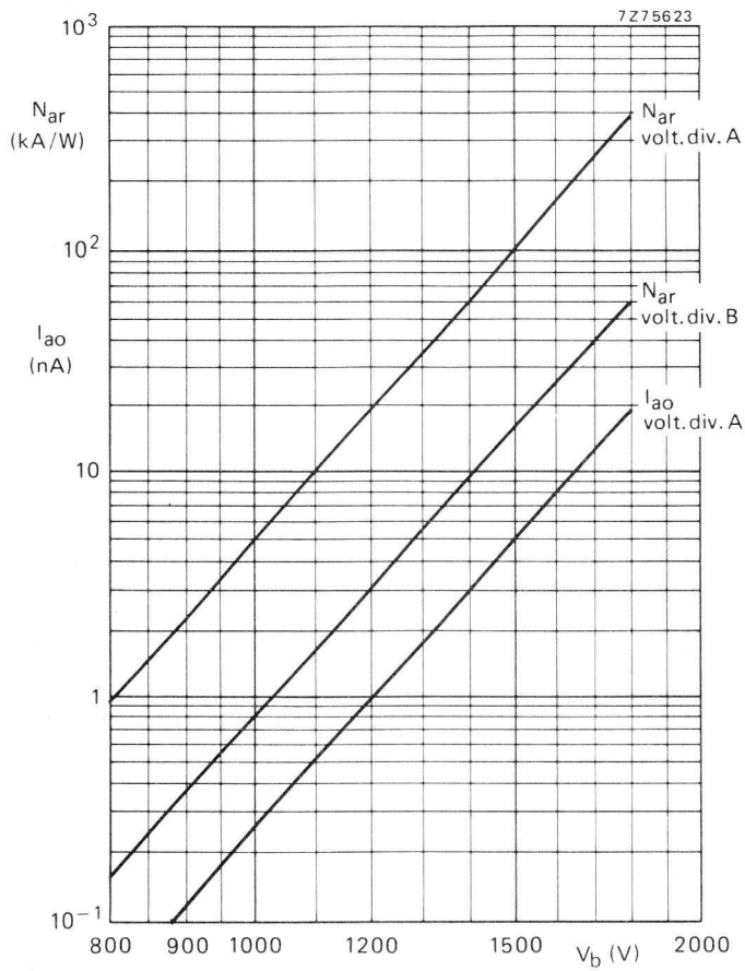
Fig. 10 Anode luminous sensitivity N_a , and anode dark current I_{a0} as a function of the supply voltage V_b .
