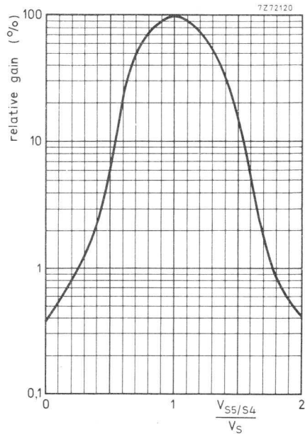
Fig. 8 Relative gain as a function of the voltage between S_5 and S_4 normalized to V_S , V_{S6/S4} constant.
