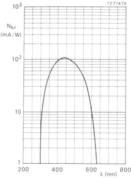
Fig. 4 Spectral sensitivity characteristic.
