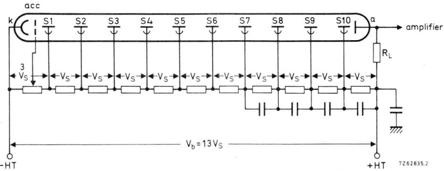
Fig. 2 Voltage divider A-1. Typical values of capacitors: 10 nF; k = cathode; acc = accelerating electrode; S_n = dynode no.; a = anode; R_L = load resistor. The accelerating electrode potential should be adjusted for optimum pulse amplitude resolution.
