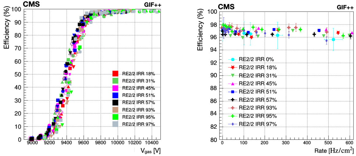
Figure 69. Left: irradiated RE2/2 chamber efficiency as a function of V_{\text{gas}} for different background irradiation rates, up to 600 Hz/cm 2 , and different integrated charge values. Different marker shapes of the same color represent different background rates at the same integrated charge values. Right: irradiated RE2 chamber efficiency at the WP as a function of the background rate at different values of the collected integrated charge. Reprinted from [129], Copyright (2023), with permission from Elsevier.
